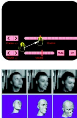
Figure 5: The scheme for head tracking shown here is based on template matching [1]. At initialization time, a frontal image of the subject is registered to a generic 3D model of the human head, and synthetically generated templates showing the appearance of the subject for a range of head poses are computed and stored. Subsequent head motion is determined by matching incoming images of the subject to the templates. The system achieves frame-rate performance by operating on subsampled images (32x32 resolution as shown in the figure). The approach is robust to non-rigid motion of the face (eyes closing, mouth opening etc).
