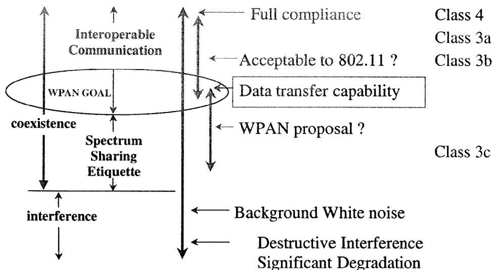
Figure 1: Coexistence/Interoperability Continuum
